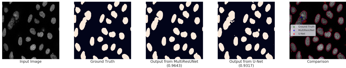
Figure 10: Segmenting images containing outliers. In the fluorescence microscopy images, there exist some bright particles, visually very similar to the cell nuclei under analysis. Although MultiResUNet can identify and reject those outliers, U-Net seems to have misclassified them.
