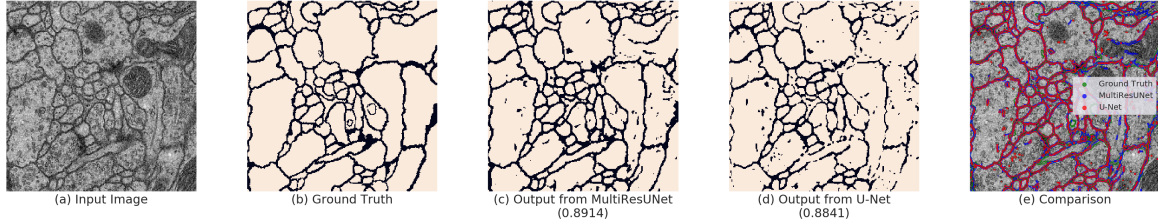
Figure 11: Segmenting the Majority Class. Here we can observe that the region of interest comprises most part of the image. Despite the values of Jacard Index for both U-Net and MultiResUNet are quite similar, visually the segmentation mask are very different. It can be seen that segmentation mask generated from MultiResUNet captures most of the fine separating lines, but U-Net tends to miss them. Moreover, there are some clusters of background pixels which although are missed by U-Net, have been roughly identified by MultiResUNet. Since the class being segmented is the majority class, the values of Jacard Index are inflated.
